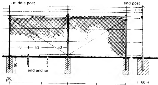
⑦ Tensioning of intersecting wire netting
